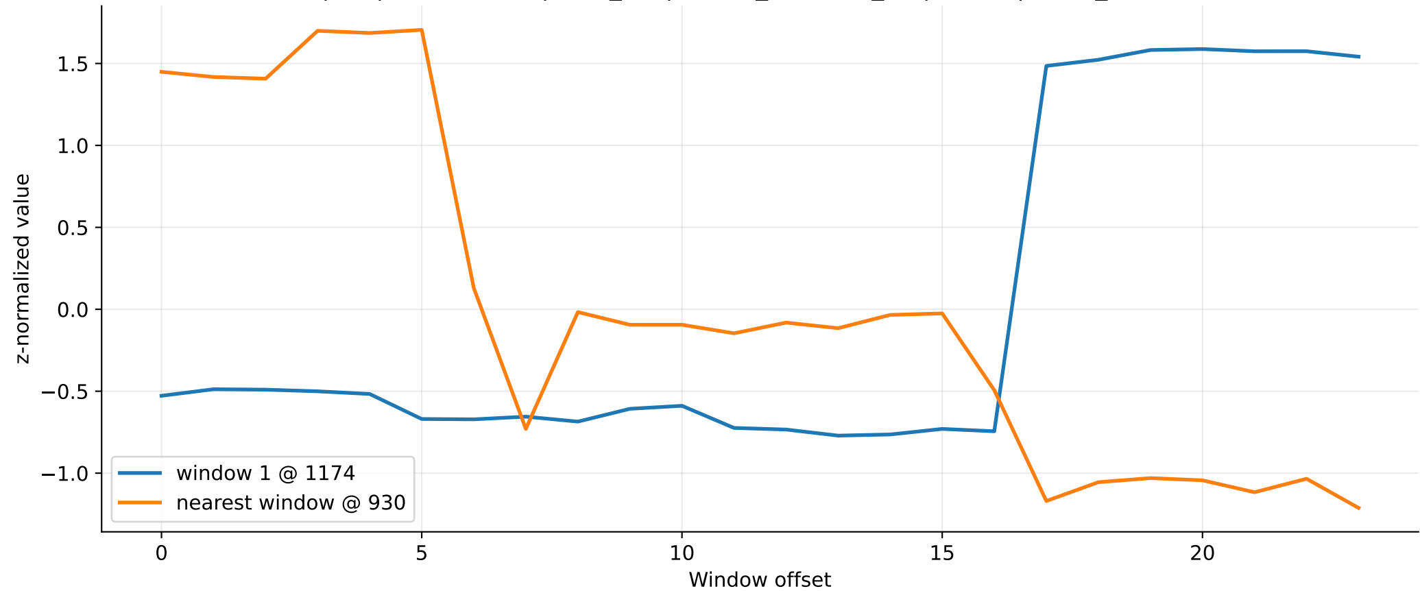
BTCUSDT | 1h | conditioned | high_vol | rolling_volatility_60 | w=24 | motif_distance=0.1895
